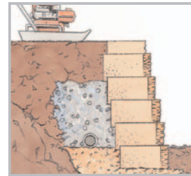
Dia. 8 – Finish Grade
