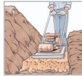
Dia. 2 – Leveling Pad
