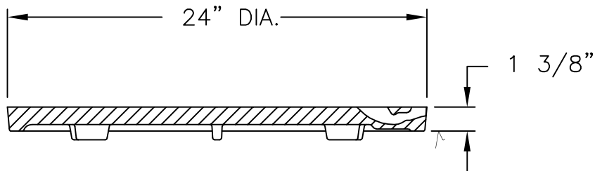
SECTION VIEW
